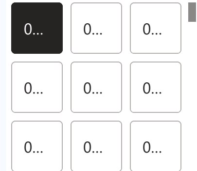
InvoiceDate
